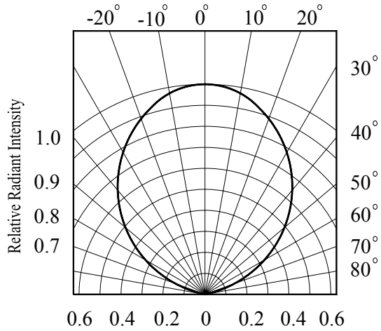
Fig.5 Relative Radiant Intensity vs. Angular Displacement
